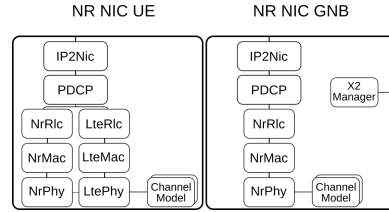
Figure 3: NIC modules
