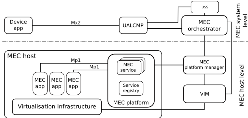
Figure 1: MEC architecture
