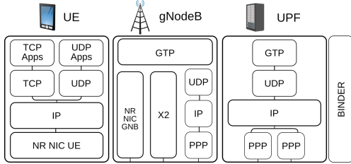
Figure 2: Simu5G main modules
